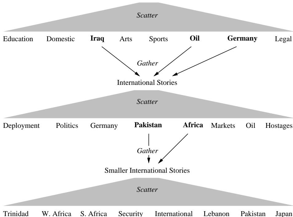
Figure 1: Illustration of Scatter/Gather
